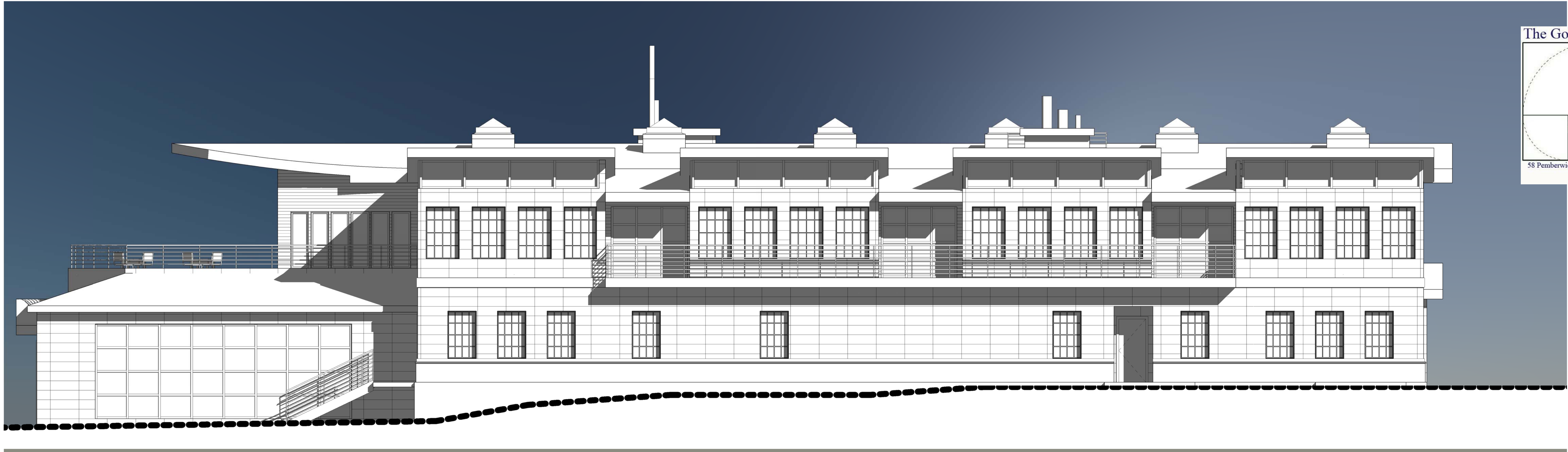
① South 3/16" = 1'-0"
